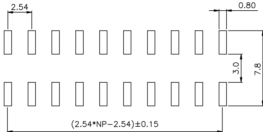
PCB LAYOUT
