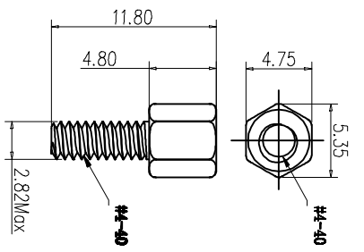
Screw specification
