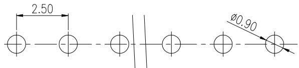
PCB LAYOUT
